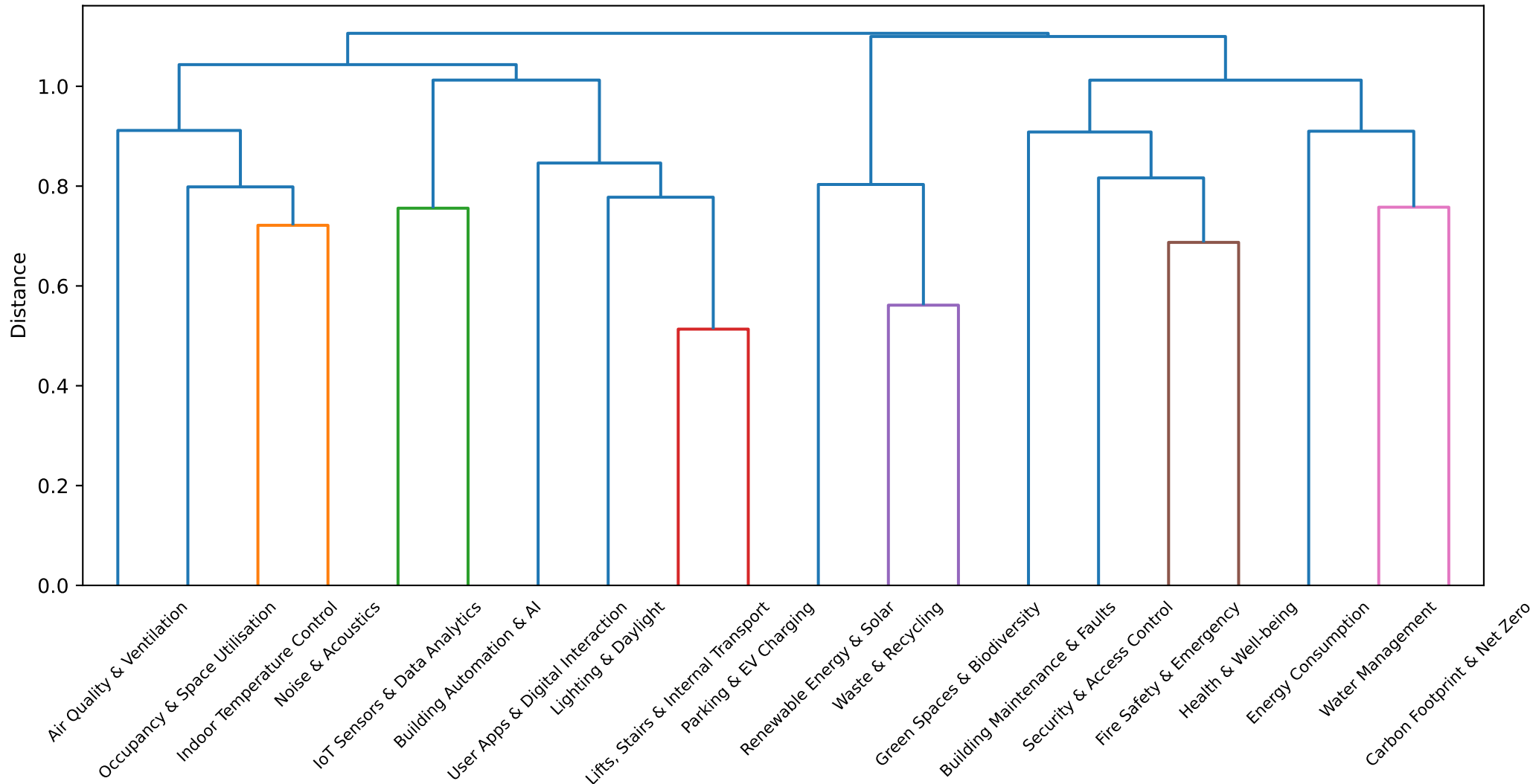
Topic clustering — average linkage on (1 - Spearman) distance
